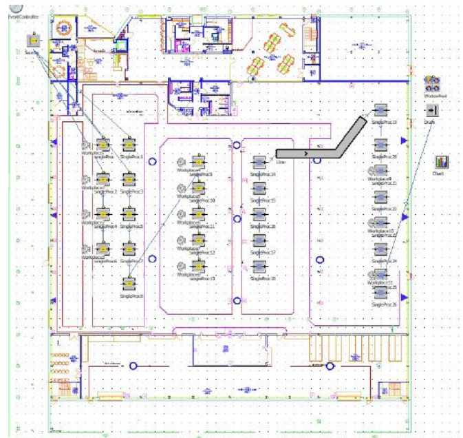
Factory flow simulation model in 2D.
